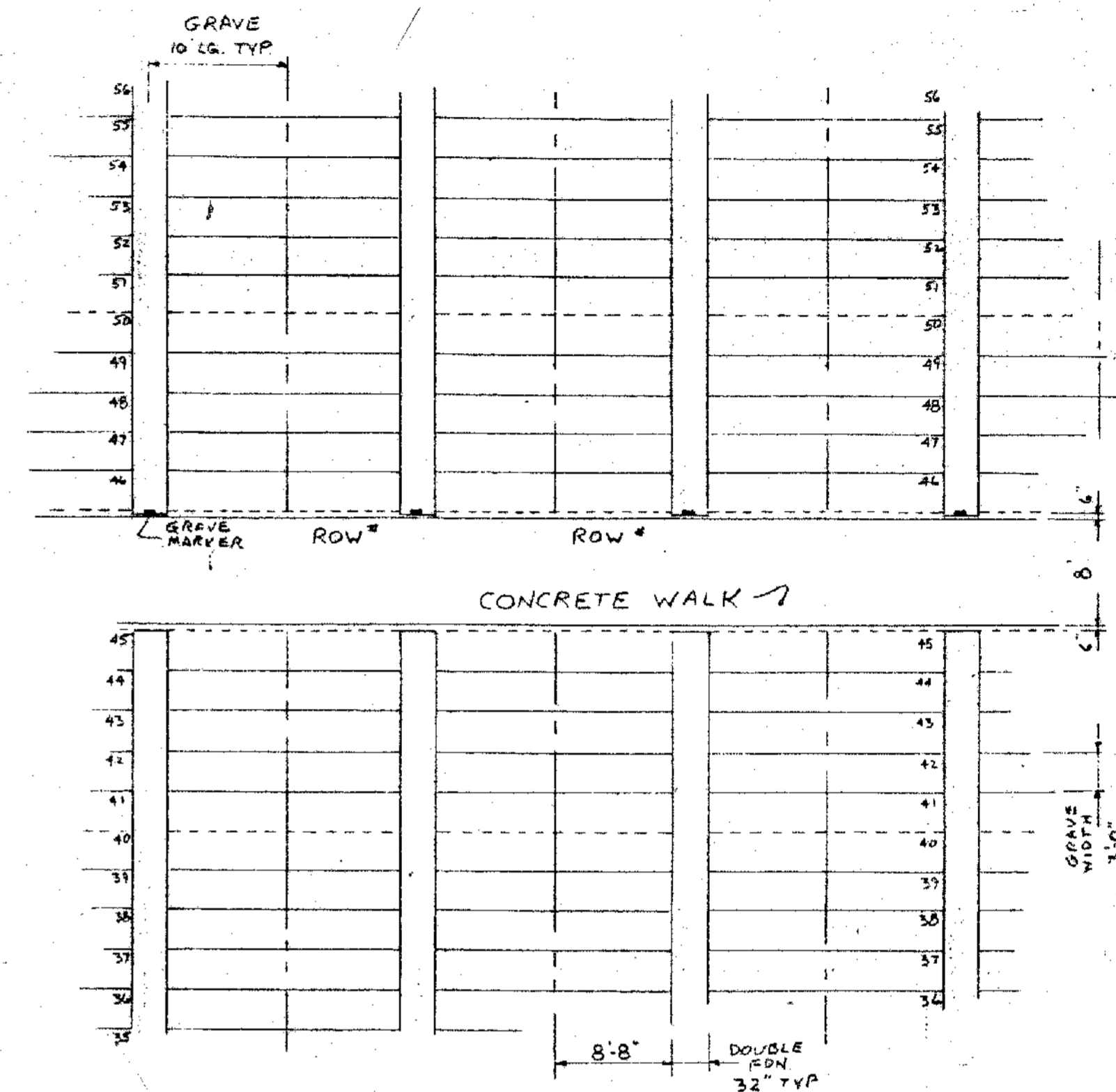
BLOW UP AT WALK SCALE: 1" = 10'
