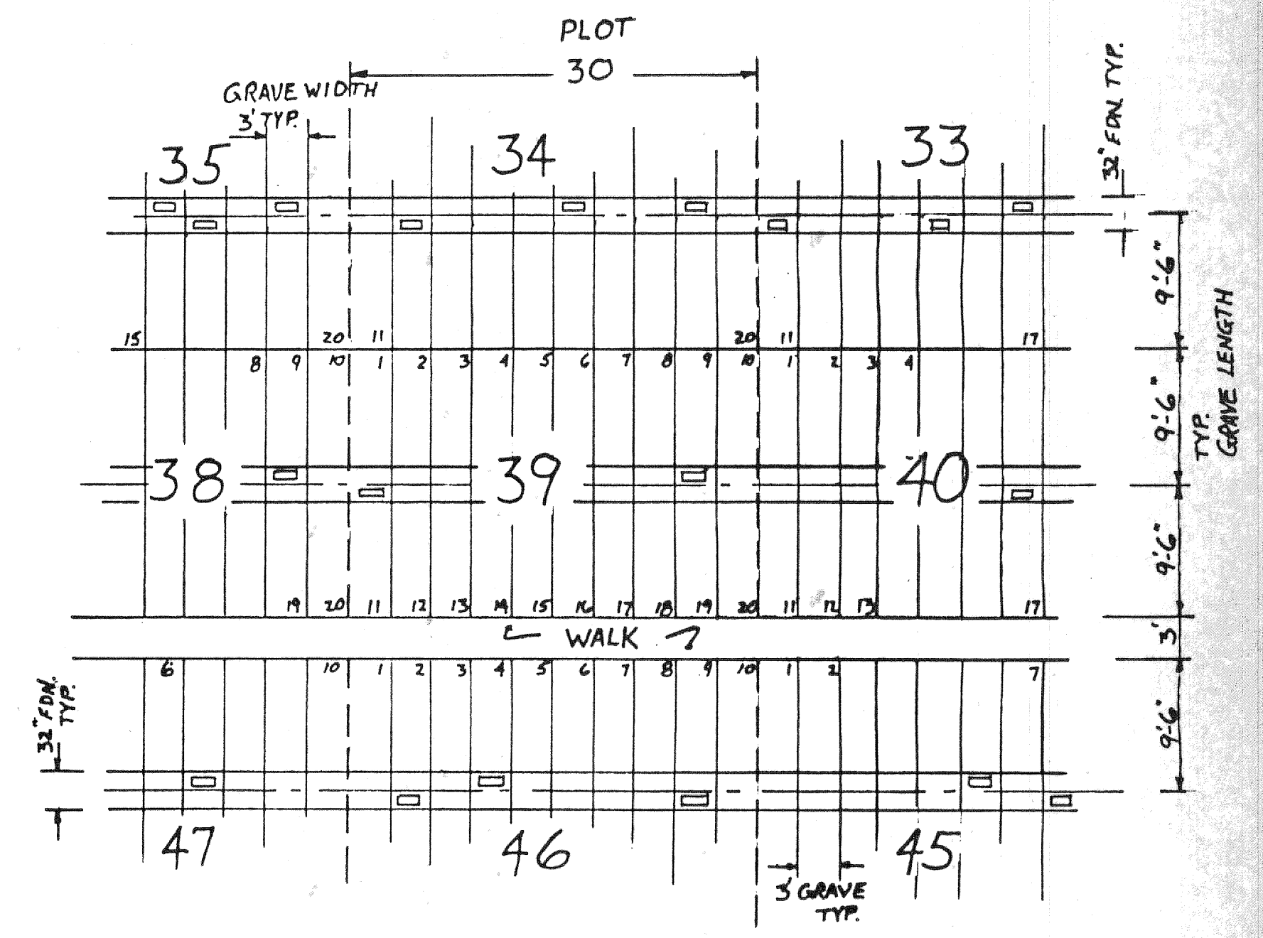
TYPICAL PLOT LAYOUT SCALE 1"=10'
