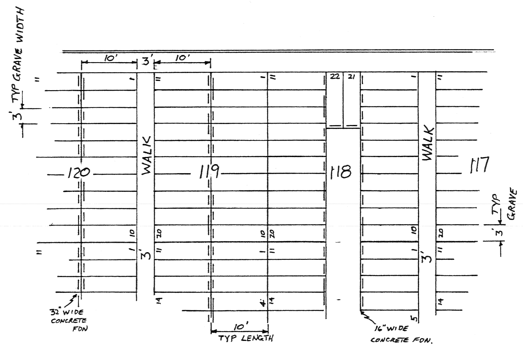
TYPICAL GRAVE SIZE & LOCATION
