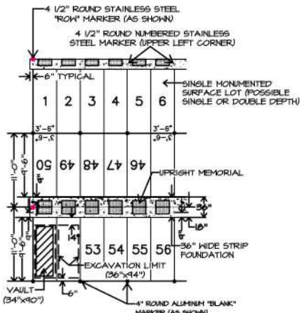
LOT LAYOUT DETAIL GRAVE SIZE: 3'-6" x 11'-0" SCALE: 1"=10'
