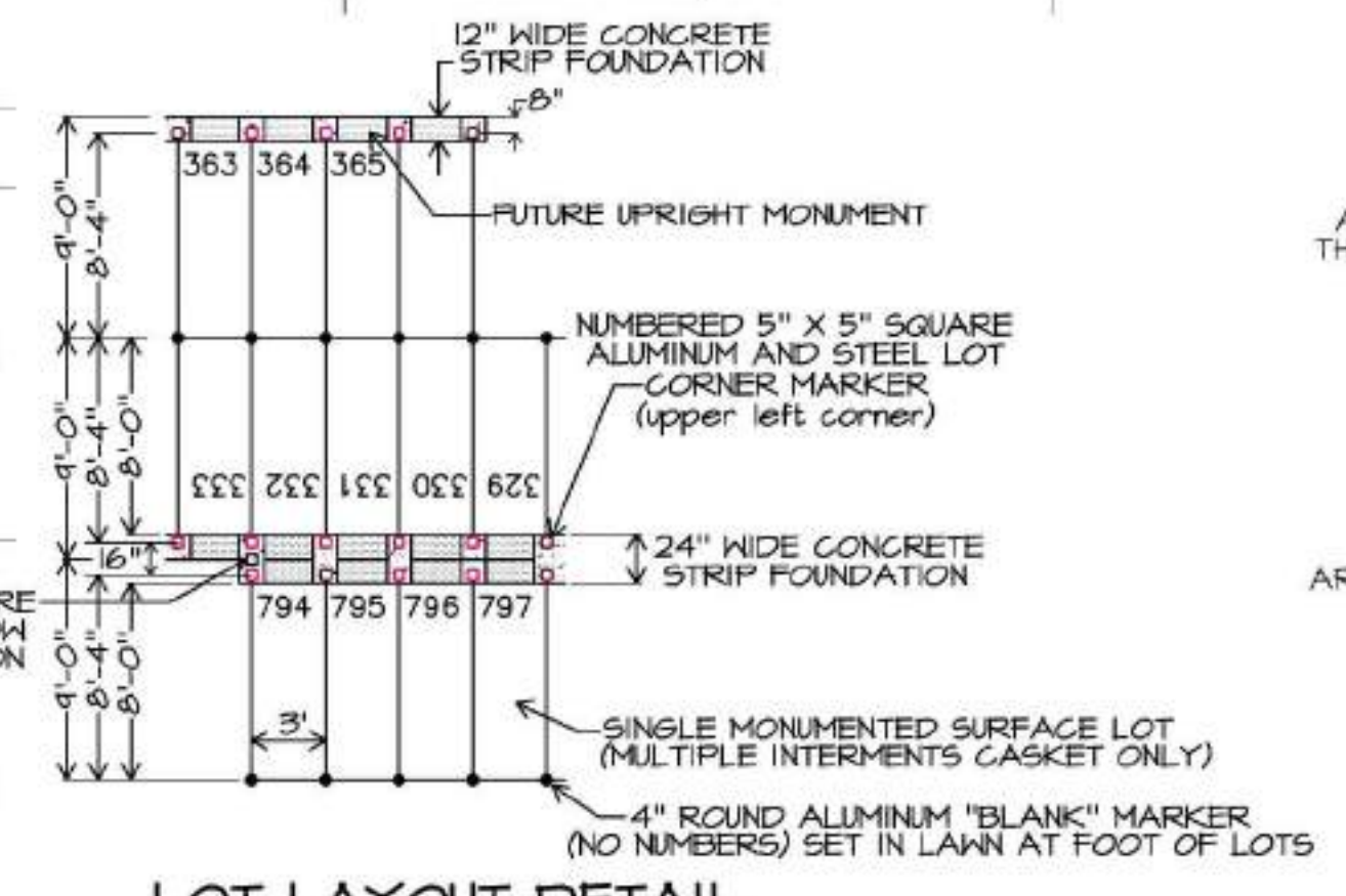
LOT LAYOUT DETAIL GRAVE SIZE: 3'-0" x 9'-0" SCALE: 1"=8'
